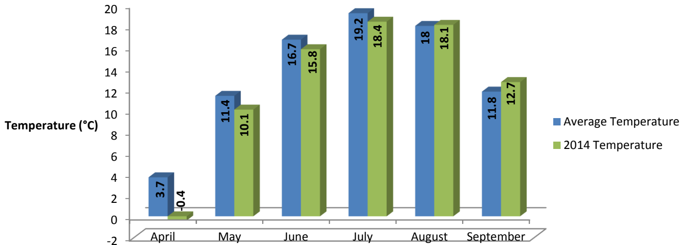
Mean Monthly Temperature vs. Average for 2014
