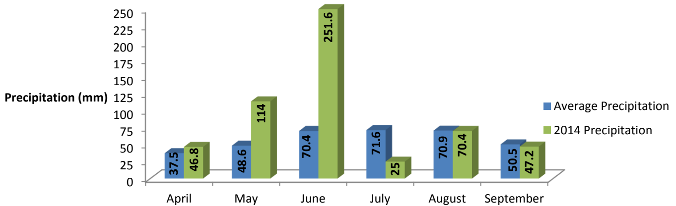
Monthly Precipitation vs. Average for 2014
